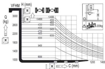
LOADING CHART 3t triplex mast
